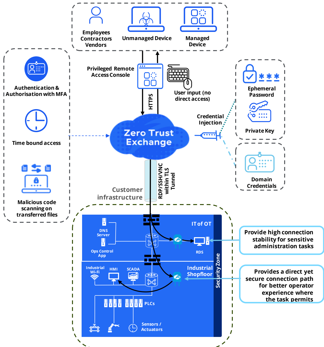
Figure 3: Conceptual architecture deployed in Case 2 using Zscaler Privileged Remote Access capability for OT Control Systems
