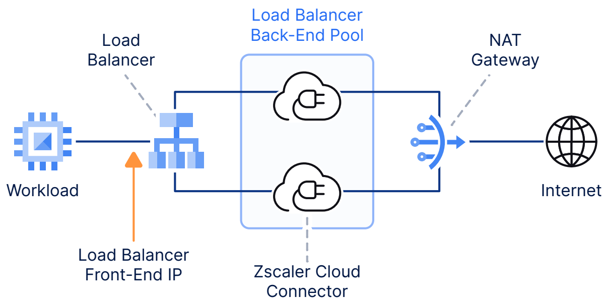
Figure 4: Cloud Connectors receive outbound traffic from the load balancer
