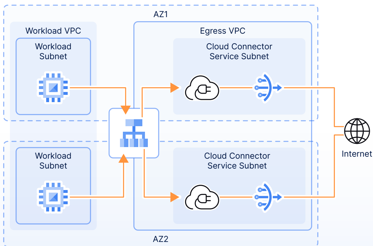
Figure 11: Deploying Cloud Connector using a Transit/Egress VPC with Shared VPC
