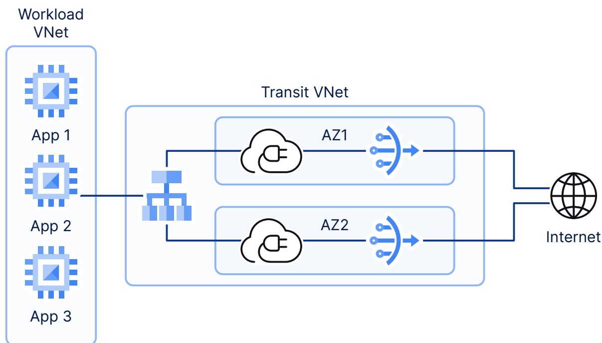
Figure 5: Cloud Connectors deployed in redundant pairs across GCP zones
