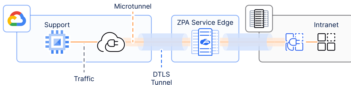
Figure 12: Cloud and on-premises workloads meet at the ZPA Service Edge
