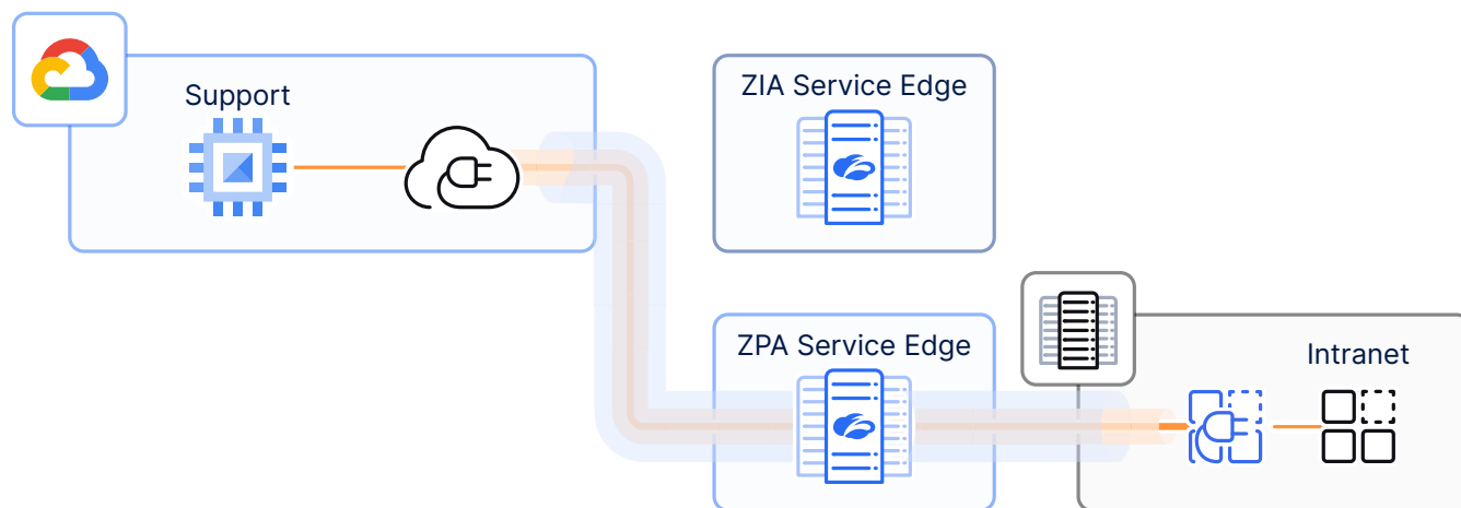
Figure 15: SIPA traffic is forwarded to a specific ZPA App Connector acting as a broker, and then goes directly to the service
