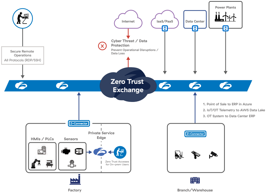
Figure 22: Zero trust for the IoT/OT systems across common access requirements.
