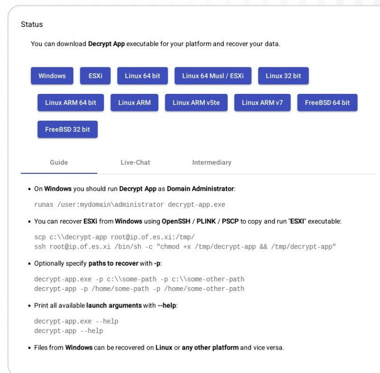
Figure 18: BlackCat/ALPHV decryption tools spanning 11 different platforms
