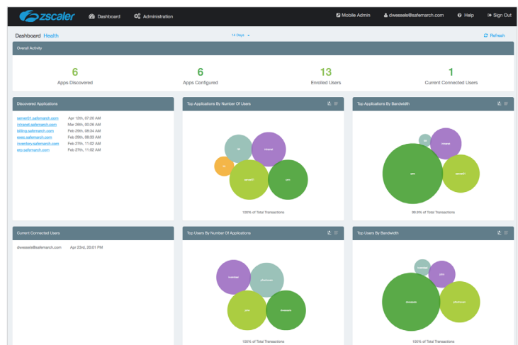
Zscaler App
